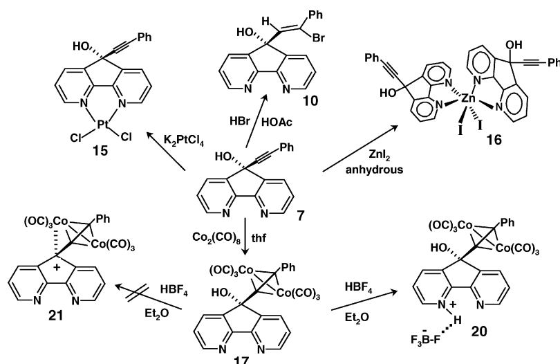
Scheme 4. Reactions of 9-phenylethynyl-4,5-diazafluoren-9-ol ( 7 ).
