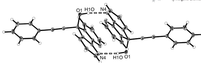
Figure 2. The \text{OH}\cdots\text{N} hydrogen bonding in 9-phenylethynyl-4,5-diazafluoren-9-ol ( 7 ).
