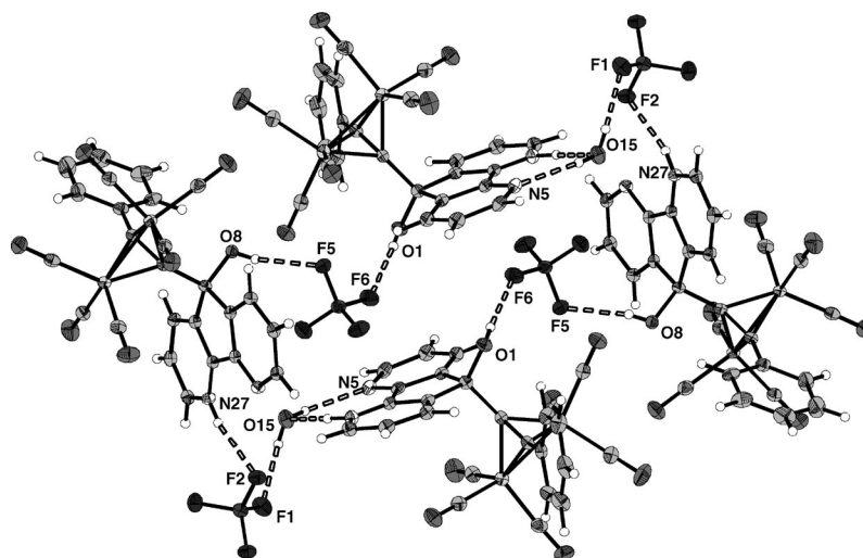
Figure 12. Structure of the alkynylpyridinium-dicobalt hexacarbonyl cluster 20 , illustrating the hydrogen bonding through the tetrafluoroborate groups and water molecules in the tetrameric assembly.
