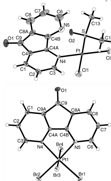
Figure 9. Molecular structures of [(dafone)PtCl 2 (dmsO)] ( 13 ) and (dafone)PtBr 4 ( 14 ).
