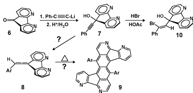
Scheme 2. Potential route to tetraazatetracenes 9 .
