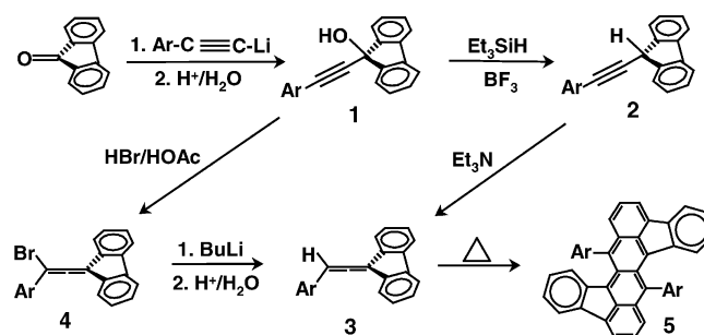
Scheme 1. Synthetic routes to diindenotetracenes 5 .
