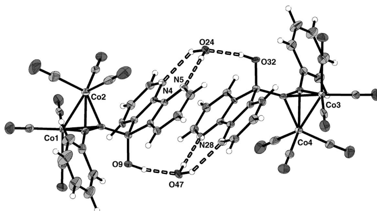
Figure 11. Structure of the cobalt cluster 17 illustrating the hydrogen bonding in the dimer, which is mediated by bridging water molecules.
