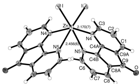
Figure 8. Molecular structure of cis -(dafone) 2 ZnI 2 ( 12 ).
