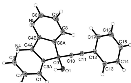
Figure 1. Molecular structure of 9-phenylethynyl-4,5-diazafluoren-9-ol ( 7 ).
