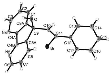
Figure 4. Molecular structure of Z-9-[(2-bromo-2-phenyl)ethenyl]-4,5-diazafluoren-9-ol ( 10 ).
