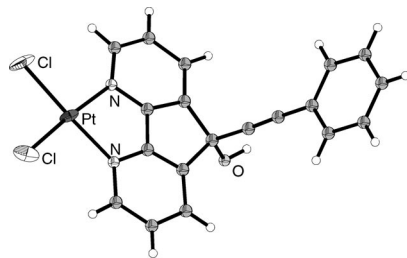
Figure 10. Structure of dichlorido(9-phenylethynyl-4,5-diazafluoren-9-ol)platinum(II) ( 15 ).
