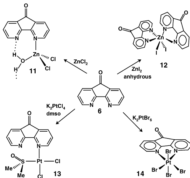
Scheme 3. Reactions of dafone ( 6 ) with metal salts.
