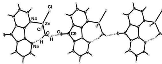
Figure 6. Bird's eye view of the hydrogen-bonding pattern in [(\text{dafone})\text{ZnCl}_2(\text{H}_2\text{O})] ( 11 ).
