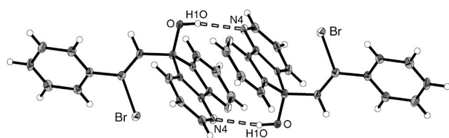
Figure 5. The intermolecular OH...N hydrogen bonding in 10 .
