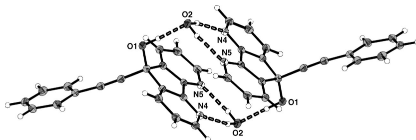
Figure 3. The hydrogen-bonding motif in 9-phenylethynyl-4,5-diazafluoren-9-ol ( \mathbf{7}\cdot\text{H}_2\text{O} ).
